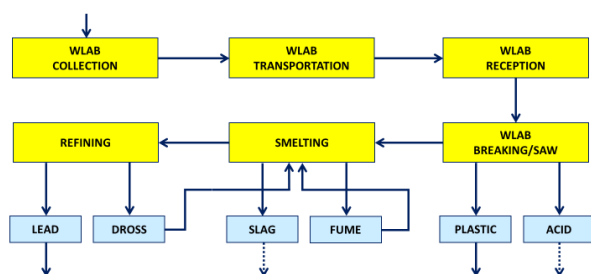
Figure 1 battery breaking and recycling processes.
