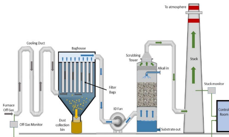
Figure 9: Flue gas desulphurisation
