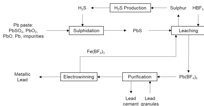
Figure 5. Diagram of FLUBOR® process.
